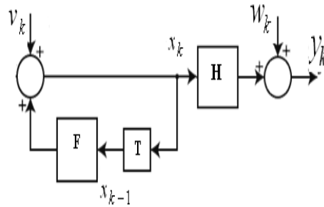
Figure1 State Space Model for Kalman Filtering Formulation
