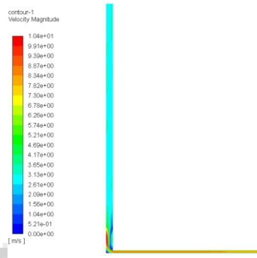
Figure 5: Velocity distribution of collector at 2 m
