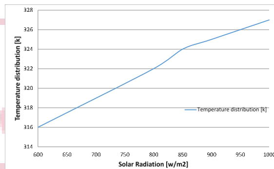
Figure 10: Temperature distribution of collector at 2 m height
