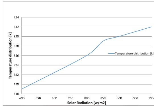
Figure 12: Temperature distribution of collector at 4 m height
