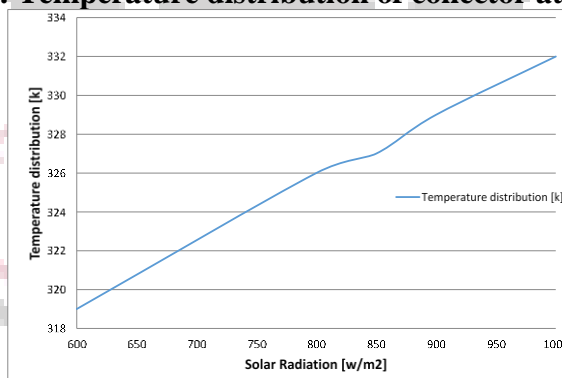
Figure 10: Temperature distribution of collector at 2 m height
