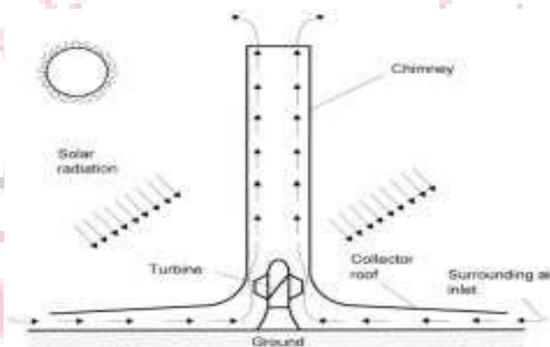
Figure 2: Solar chimney power configuration
