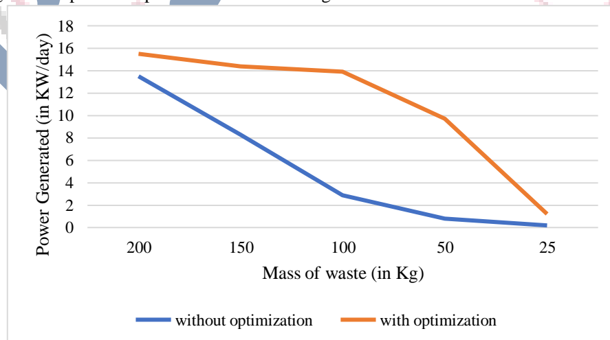
Figure 4: Power Generated with and without optimization using pig dung, chicken dung and municipal waste
