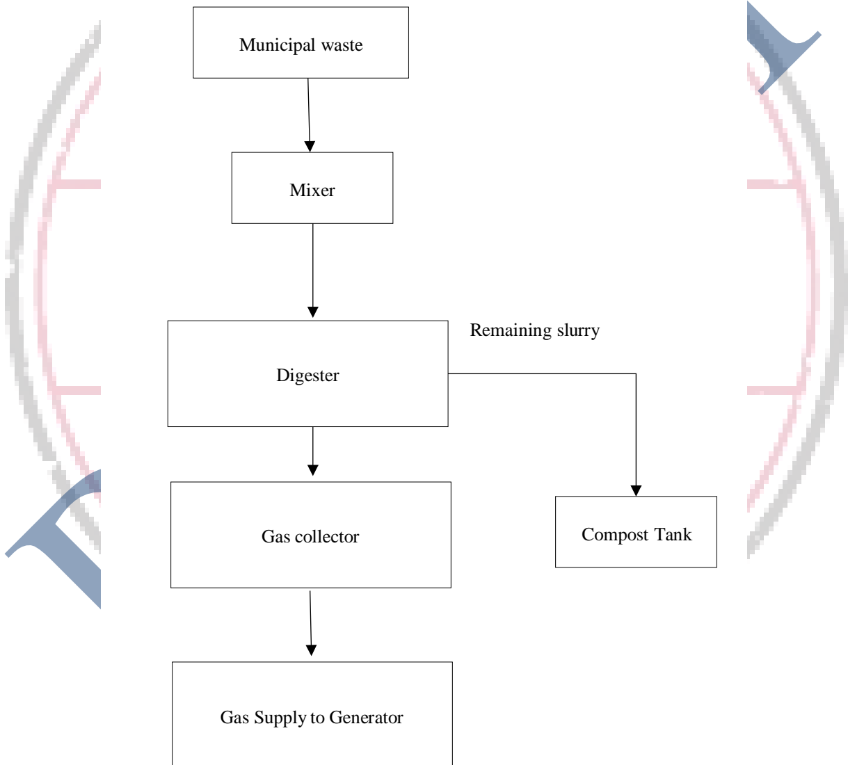
Figure 1: Flow chart of biogas production system
