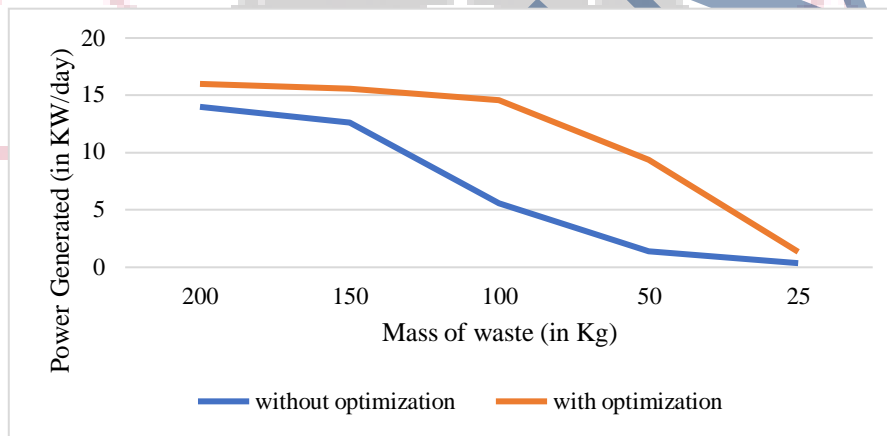
Figure 3: Power Generated with and without optimization using municipal waste
